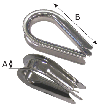
ROPE THIMBLE
