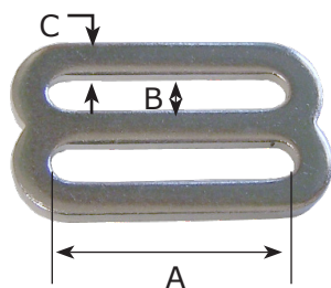
SPECIAL HEAVY SLIDE
