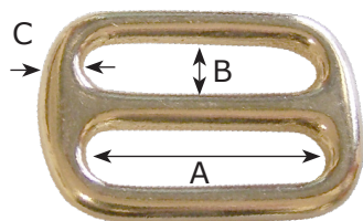
CASTED SLIDE
