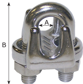
ROPE CLAMP
