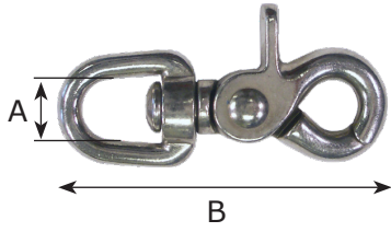
ROUND SWIVEL HEAVY TRIGGER SNAP
