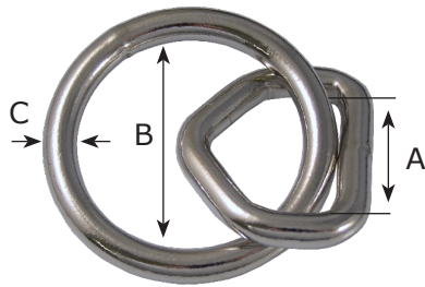
LOOP & WELDED RING
