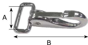
RIGID SQUARE EYE QUICK SNAP
