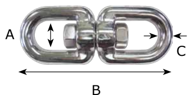
ROUND EYE DOUBLE END SWIVEL
