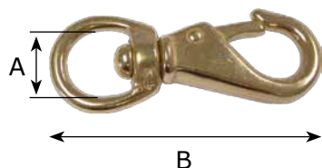
ROUND SWIVEL BOAT SNAP
