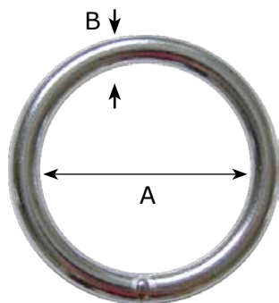
WELDED O-RING
