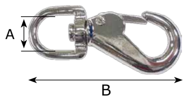
ROUND SWIVEL BOAT SNAP
