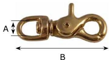
ROUND SWIVEL TRIGGER SNAP
