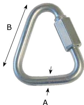
DELTA SHAPED QUICK LINK
