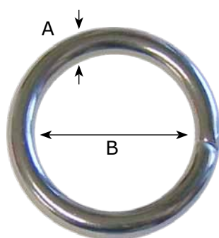
UNWELDED O-RING
