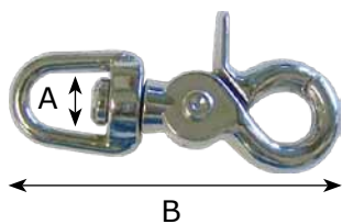
ROUND SWIVEL LIGHT BODY TRIGGER SNAP
