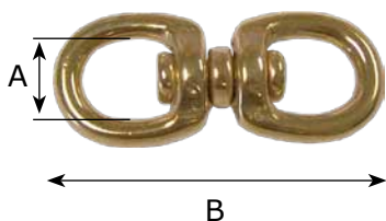
ROUND EYE DOUBLE END SWIVEL
