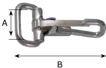
RIGID SQUARE EYE SPRING SNAP
