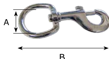
HEAVY ROUND SWIVEL BOLT SNAP
