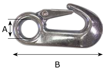
SAFETY SNAP
