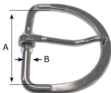
FLAT GIRTH BUCKLE
